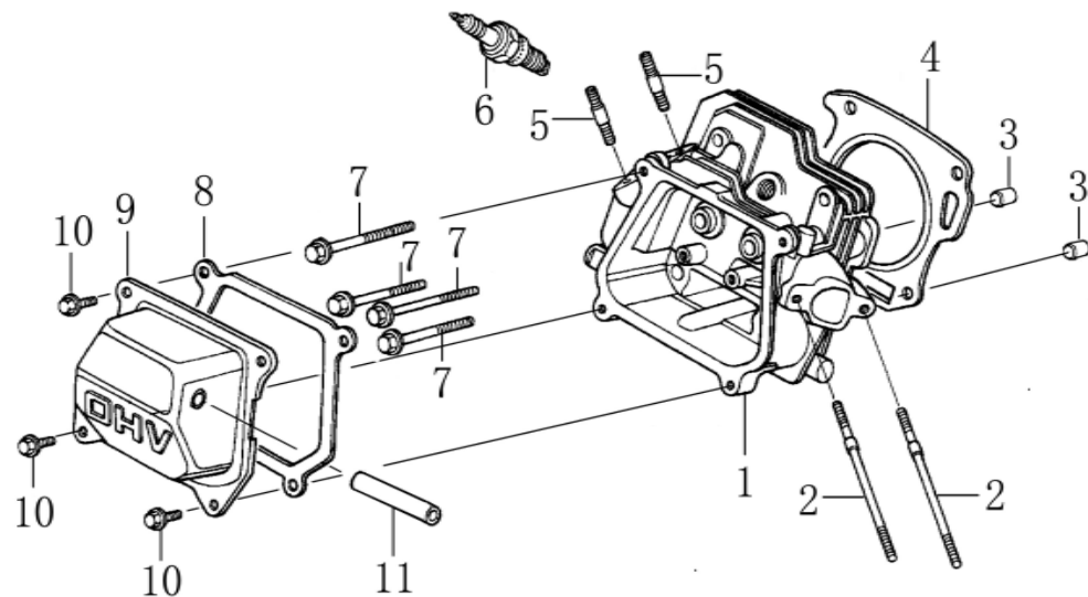
气缸头 (CYLINDER HEAD)
